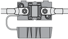
A single fuse and holder setup from the Fuse Kits available from REDARC. Part number FK40 (40 A) or FK60 (60 A).
