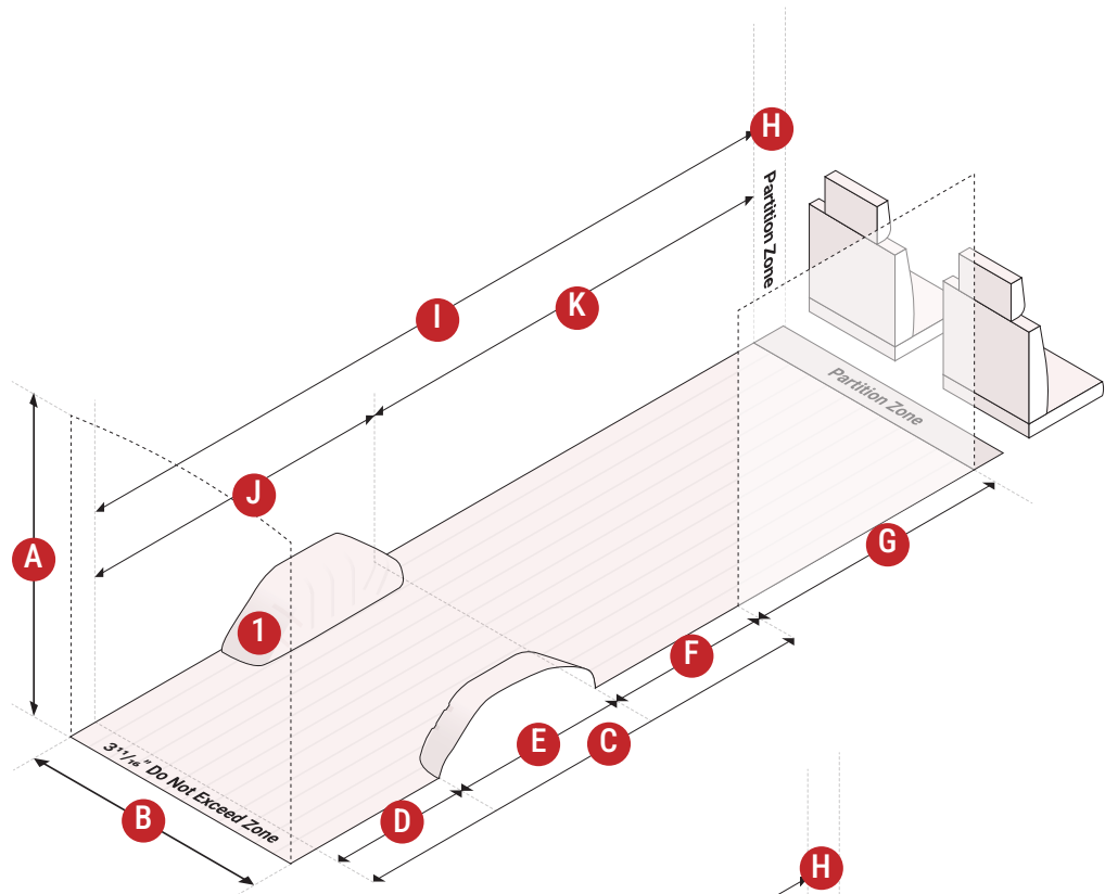
170" WB SUPER HIGH ROOF 2007-2018 SPRINTER 2500/3500
