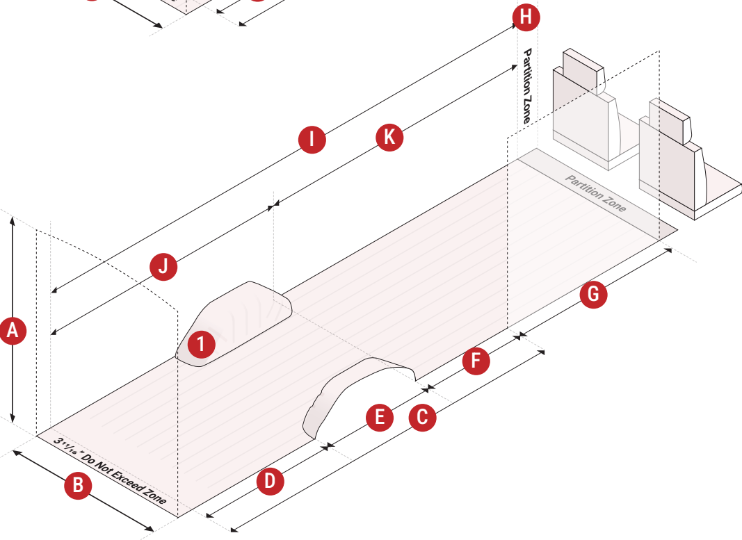
170" EWB SUPER HIGH ROOF 2007-2018 SPRINTER 2500/3500
